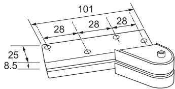
9143TC(L) Offset top centre
