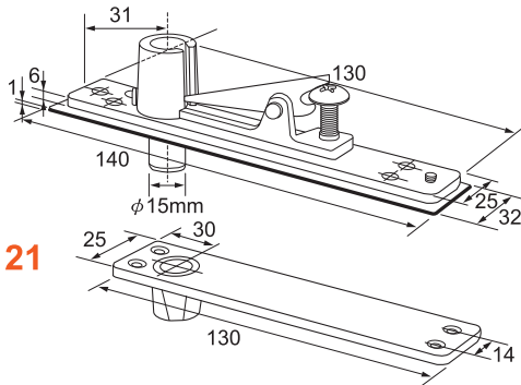
9143TC(L) Offset top centre
