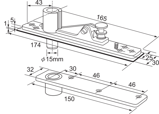
9118/9 Adjustable top centre with \phi 15mm pin
