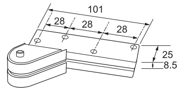
9143TC(R) Offset top centre
